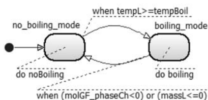
Fig. 7. B-chart for the boiling process
