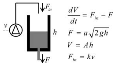
Fig. 4. Model used to illustrate run-time selection of state variables
