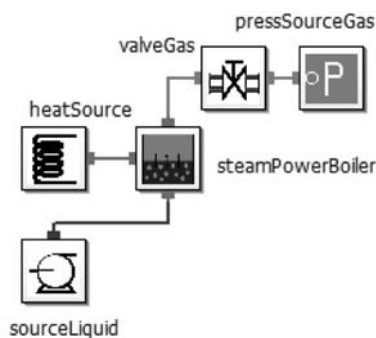
Fig. 6. Diagram of the boiler model
