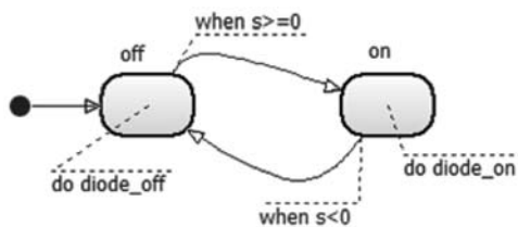
Fig. 2. B-chart describing the behavior of a diode
