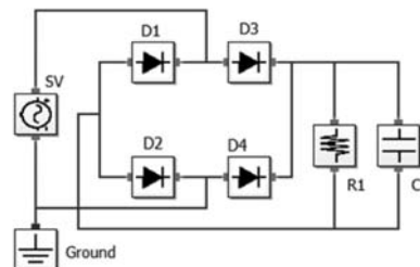
Fig. 3. Rectifier circuit model composed using RMD
