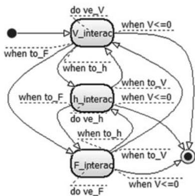
Fig. 5. B-chart of the tank system shown in Fig. 4
